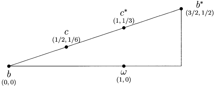
Figure 1. Counterexample to Premise 2.
